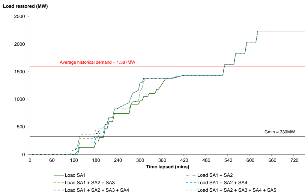
Figure 7.1: System restoration pathways - South Australia
