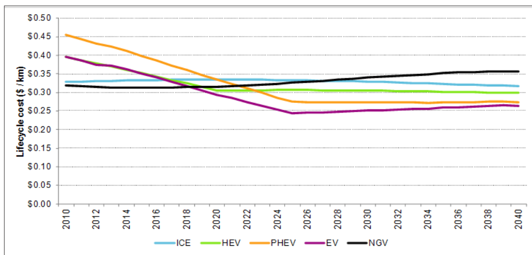
Figure 42: Lifecycle cost – medium car, high VKT
