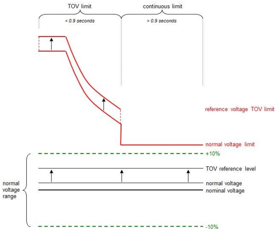
Figure 1.2 Impact of Rule change on TOV limits
