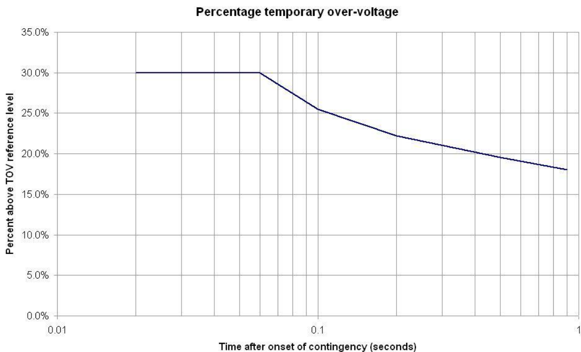
Figure 1.3 Proposed modification to Figure S5.1a.1 from the Rules
