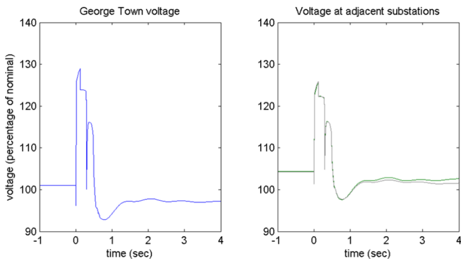
Figure 5.1 Effect of a TOV event at adjacent substations
