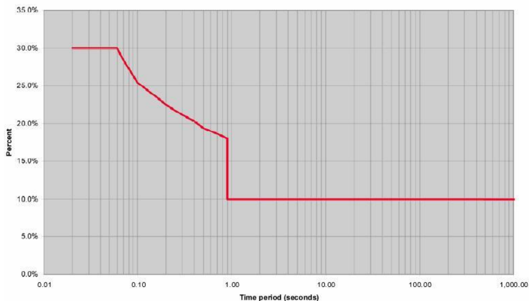
Figure 1.1 Percentage Over-Voltage - Figure S5.1a.1 from the Rules
