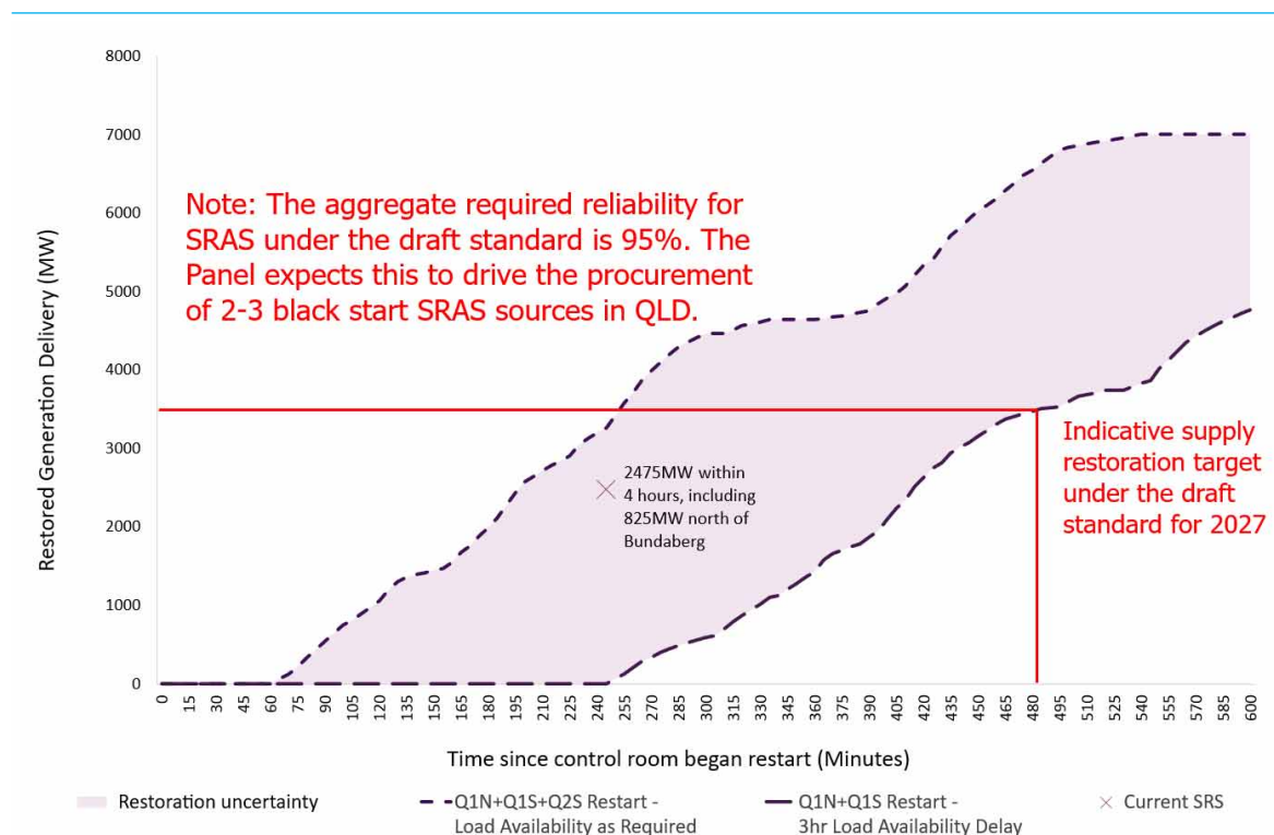
Figure A.1: Draft standard - Restoration level and time for QLD
