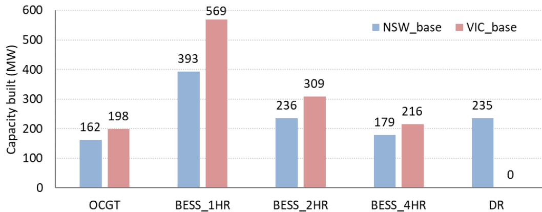
Figure 63 New entrant capacity requirements (Base case sensitivity)
