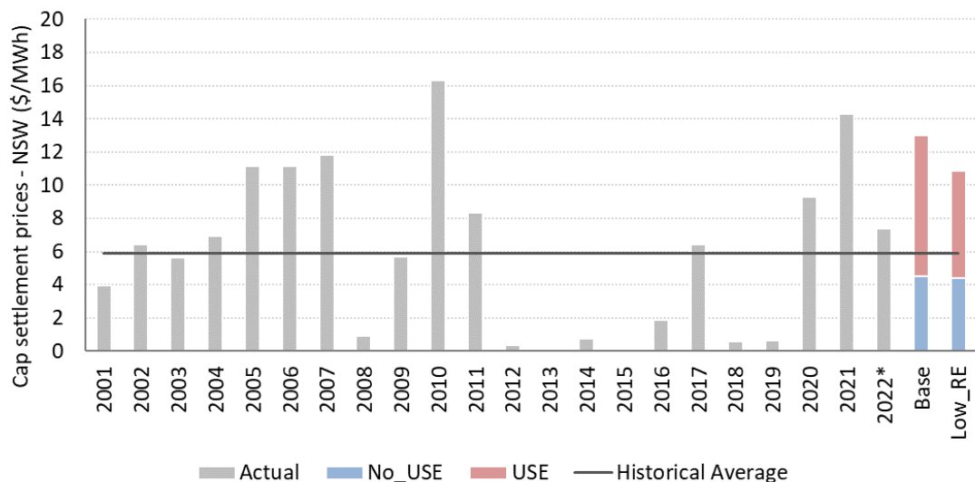
Figure 73 Modelled cap values and historical settlement (NSW)
