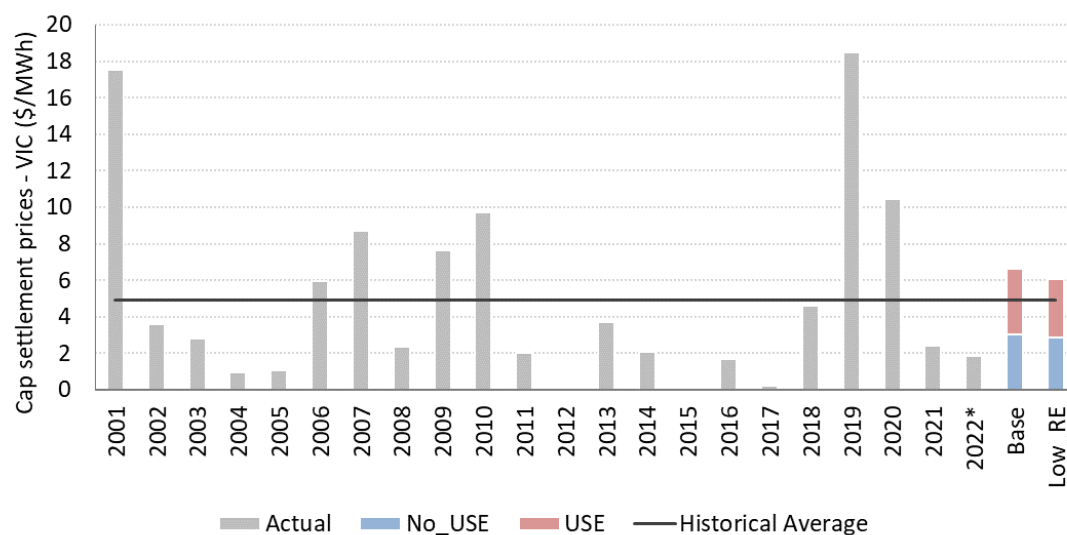
Figure 99 Modelled cap values and historical settlement (VIC)
