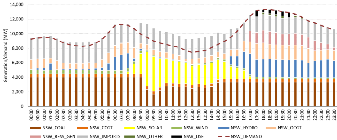
Figure 40 Snapshot dispatch profile (NSW, Low RE)
