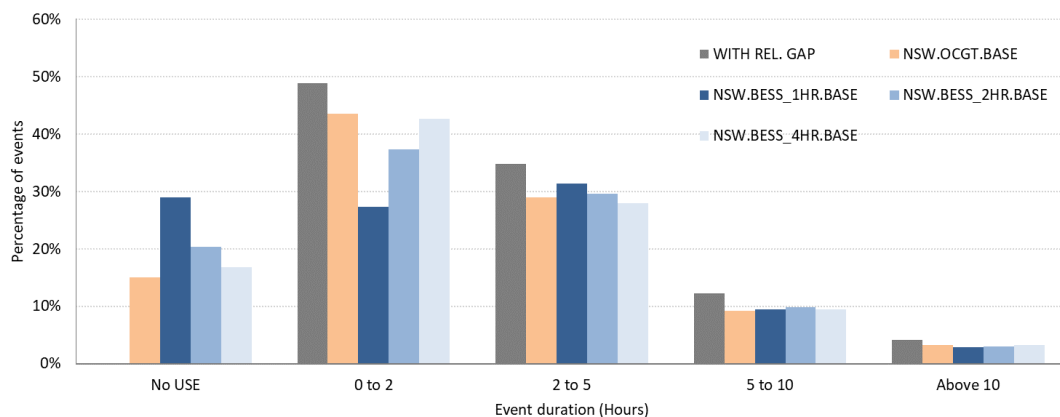
Figure 82 Distribution of event duration (NSW, Base case sensitivity)
