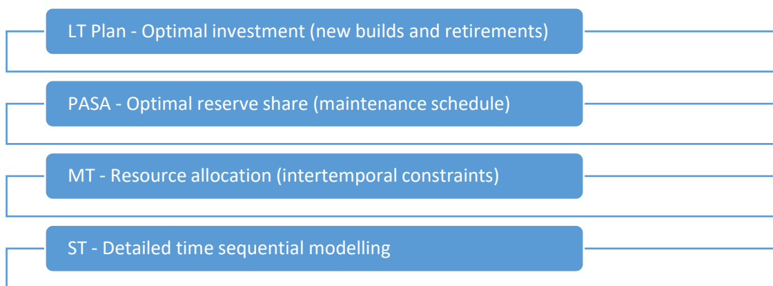
Figure 96 PLEXOS simulation phases
