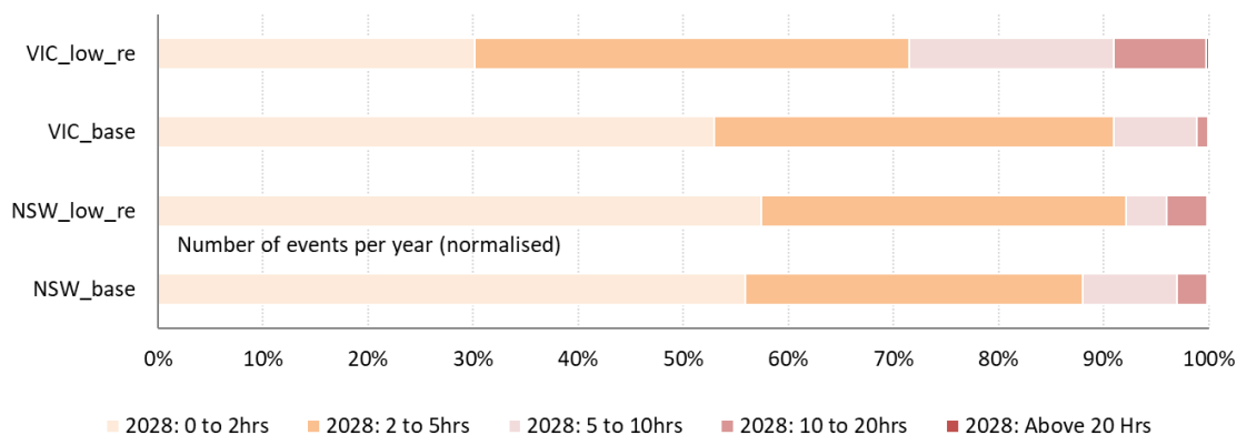
Figure 48 Expected events by event duration (normalised)
