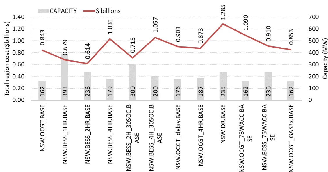
Figure 61 Results overview (NSW, Base case sensitivity)
