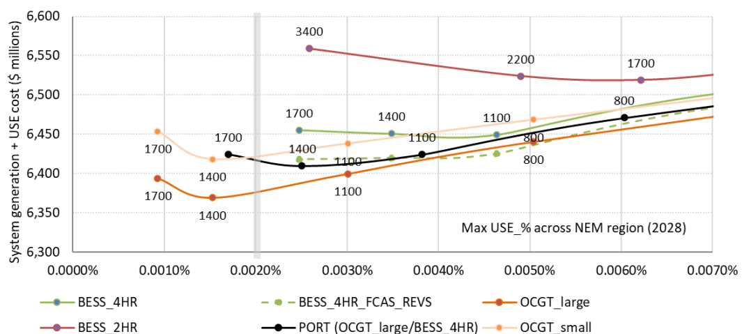
Figure 3 Task 1 - Efficiency functions (base value of customer reliability)
