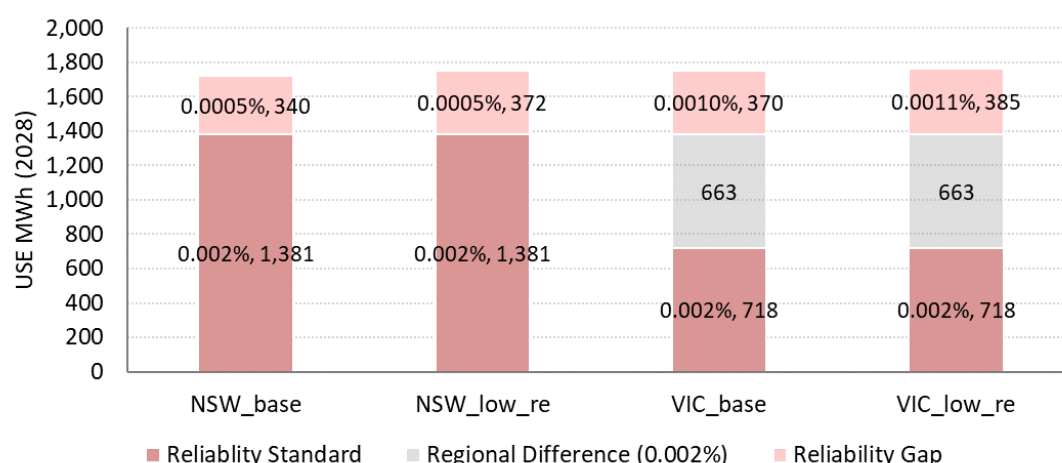
Figure 95 Base USE volume differences
