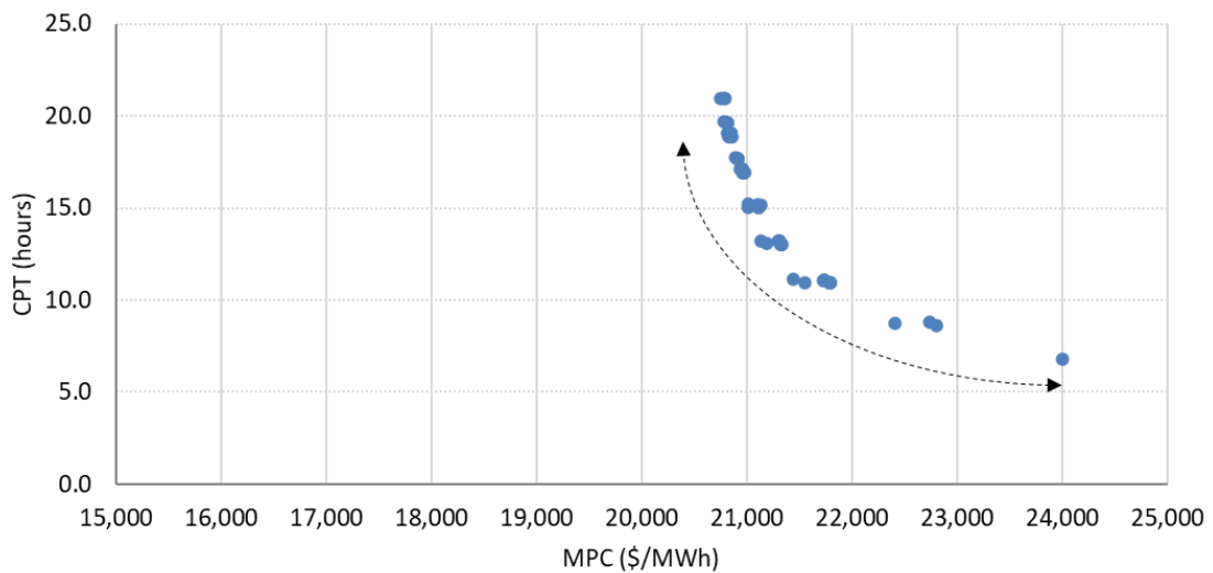
Figure 66 MPC and CPT combinations for OCGT
