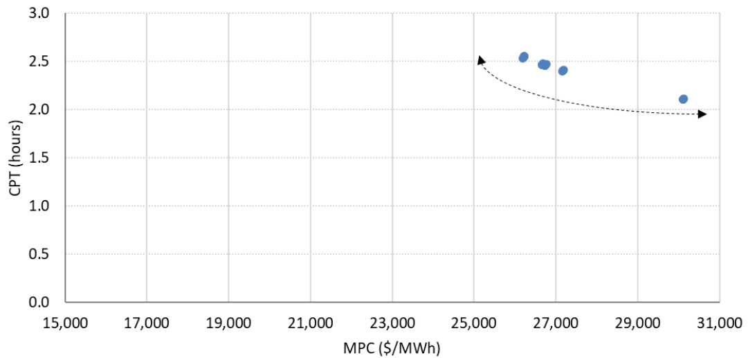
Figure 67 MPC and CPT combinations for BESS_2HR
