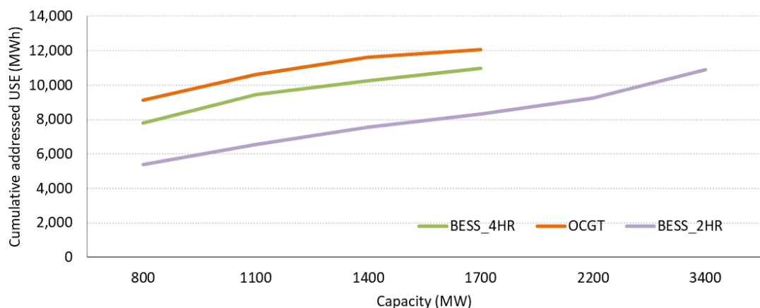
Figure 20 Cumulative addressed USE
