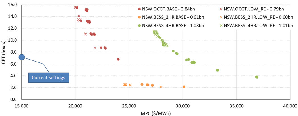
Figure 80 NSW MPC and CPT combinations (Base and Low RE)
