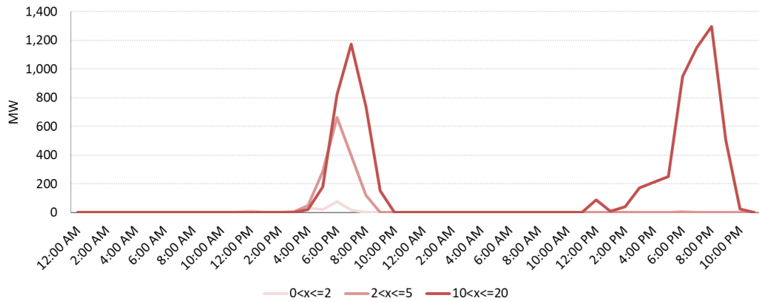
Figure 59 Daily shape by event duration (VIC, Low RE scenario)
