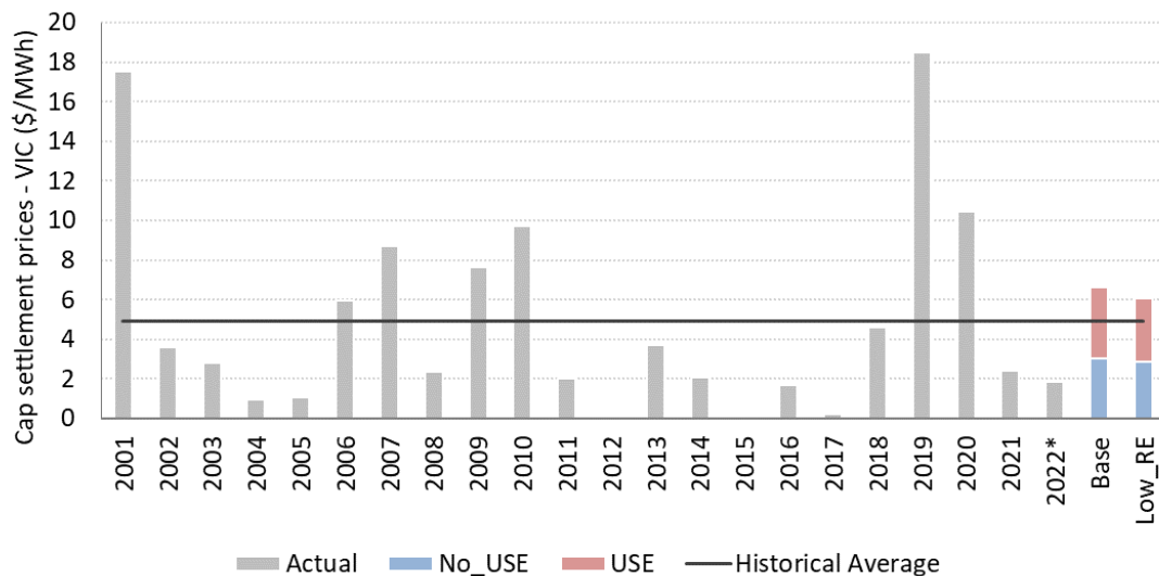
Figure 74 Modelled cap values and historical settlement (VIC)
