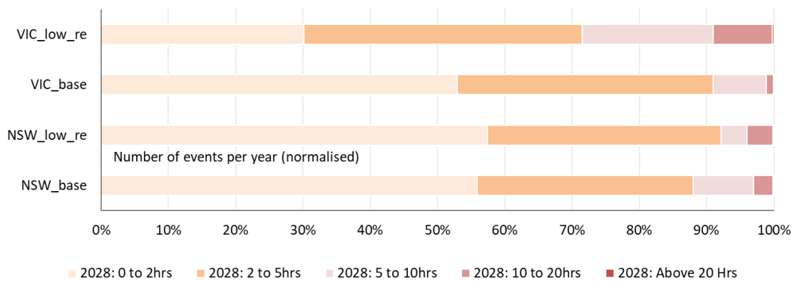
Figure 5 Task 2 - Expected events by duration (with reliability gap, normalised)
