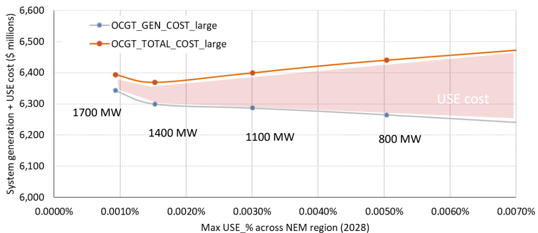
Figure 18 Total system cost components
