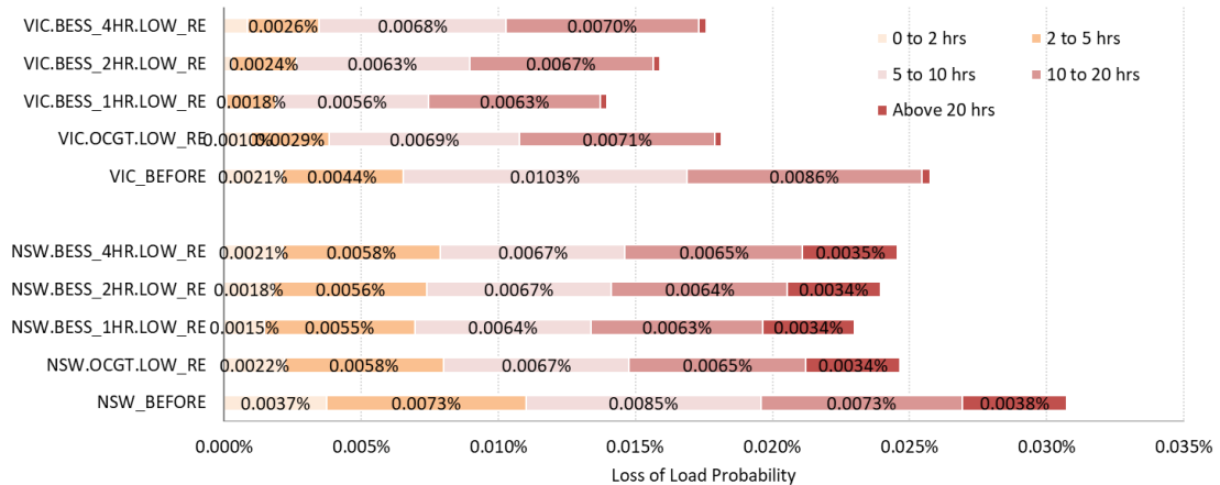
Figure 93 Loss of Load Probability (Low RE)
