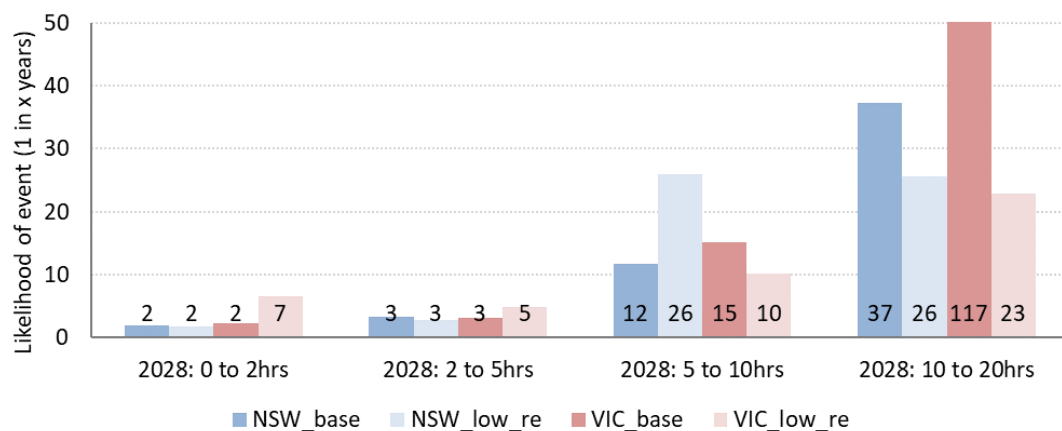
Figure 6 Task 2 - Likelihood of events by event duration (with reliability gap)
