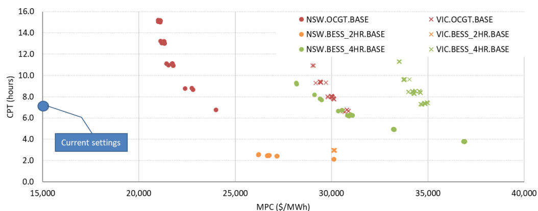
Figure 7 Task 2 – VIC and NSW baselines (Base case sensitivity)
