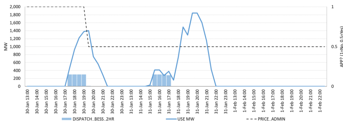
Figure 65 Dispatch chart example (BESS_2HR)
