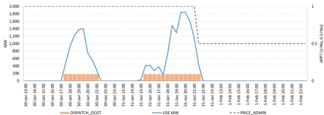
Figure 64 Dispatch chart example (OCGT)
