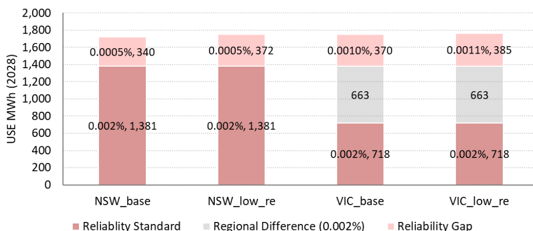
Figure 8 Task 3 - USE volume differences
