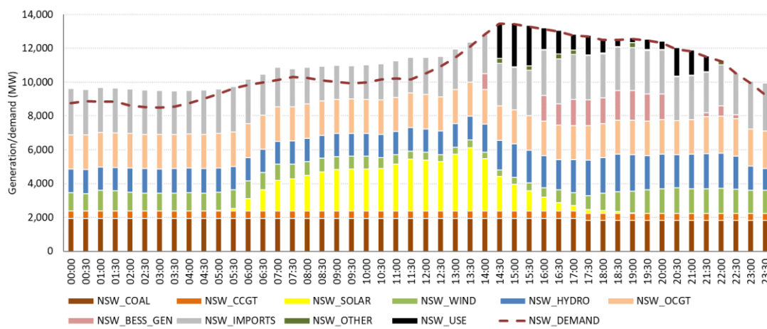
Figure 39 Snapshot dispatch profile (NSW, Base case sensitivity)
