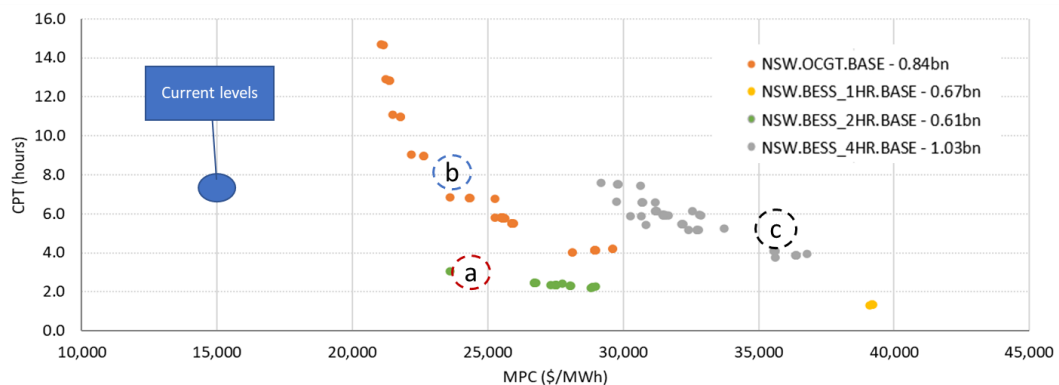
Figure 94 Considerations for MPC and CPT combination
