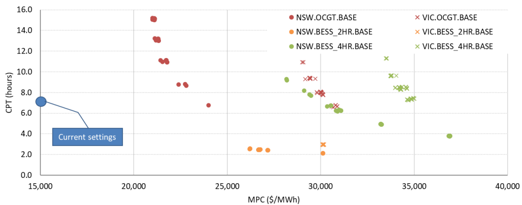
Figure 70 VIC and NSW baselines (Base case sensitivity)
