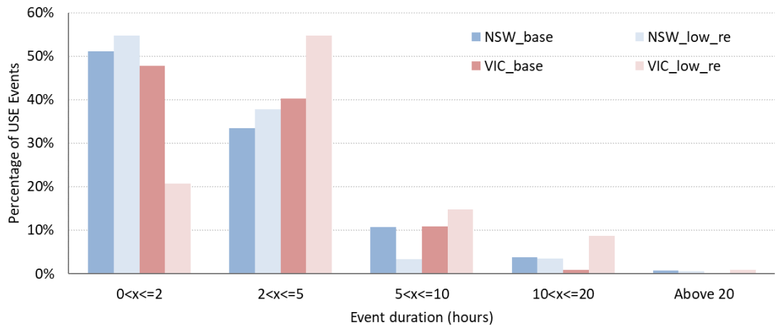
Figure 54 Distribution of event duration
