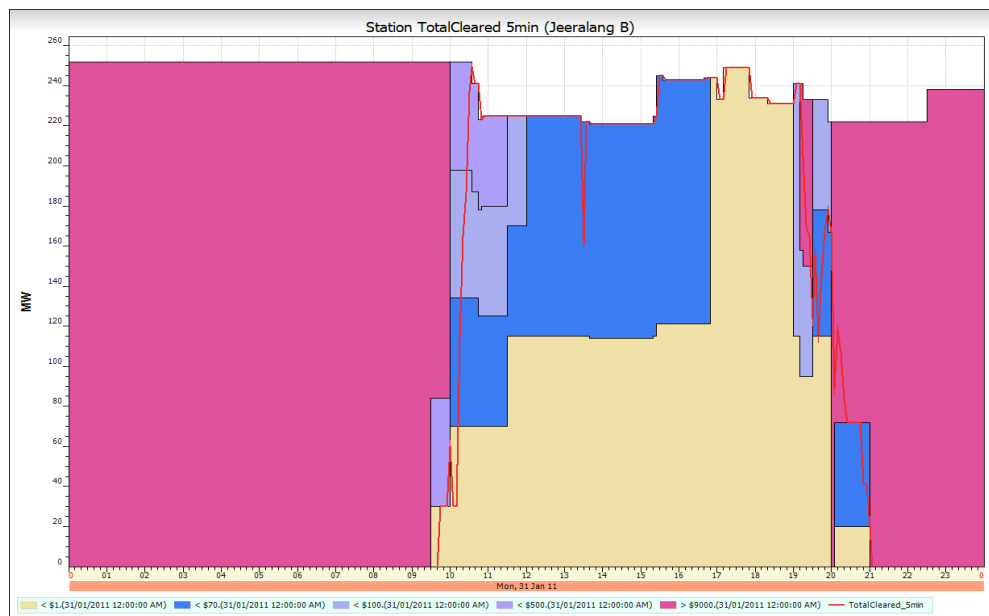
Figure 11-1 Jeeralang B Bids on a Day its Generates
