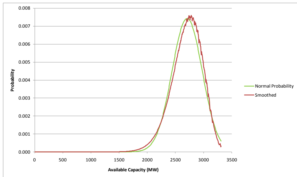
Figure 14-2 Distribution of Availability and Fitted Normal Distribution
