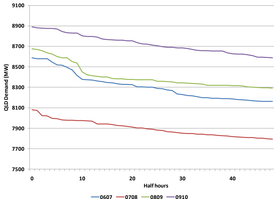
Figure 6-4 Historic Queensland Load Duration Curves (top 25 hours)
