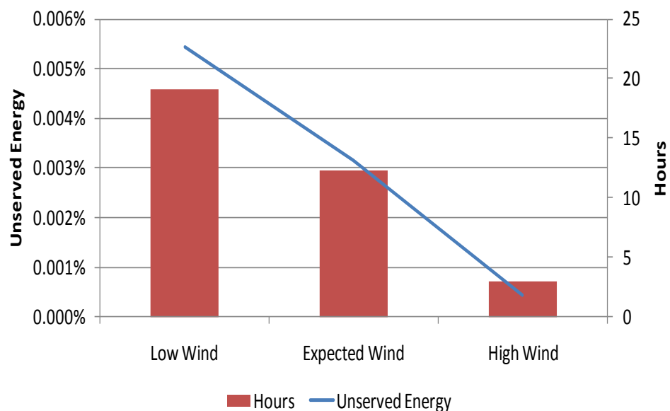
Figure 6-7 SA Reliability Sensitivity to Wind Pattern Assumed
