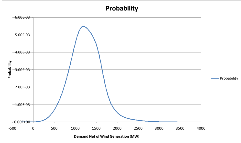
Figure 14-9 Probability Distribution of Demand – Wind Generation
