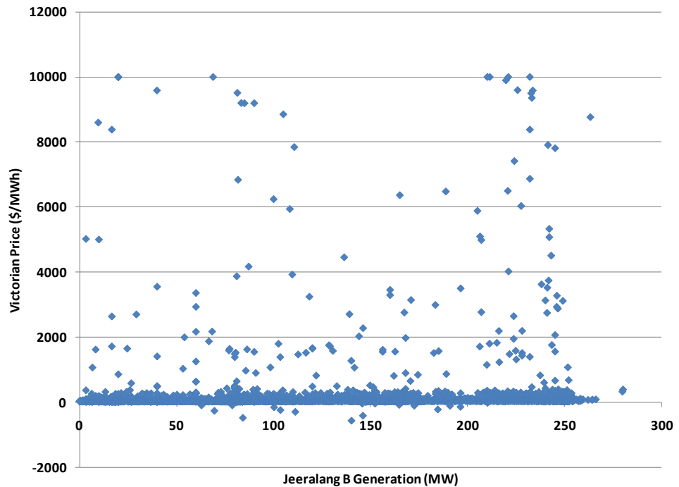
Figure 7-2 Jeeralang B Generation versus Spot Price: 2006-2011
