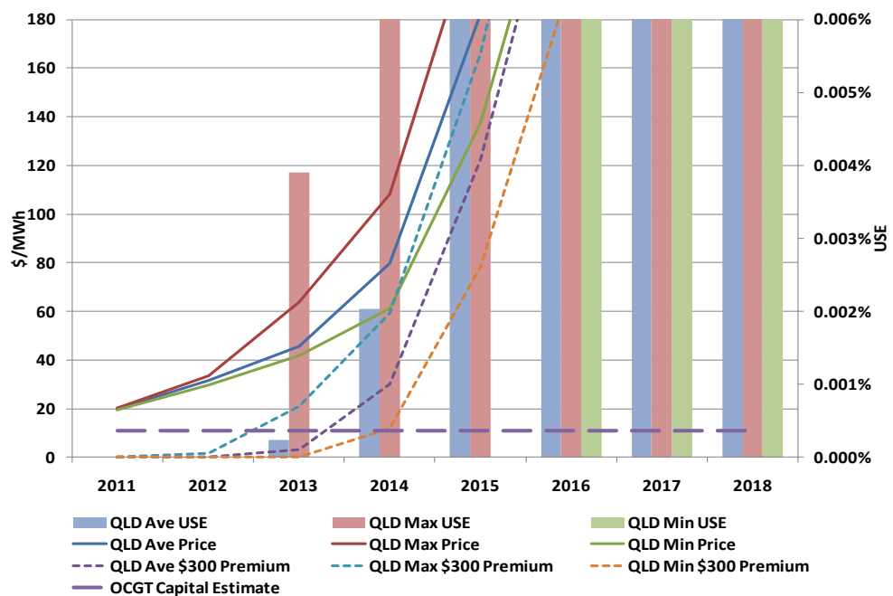
Figure 8-2 QLD 50 PoE No New Entry
