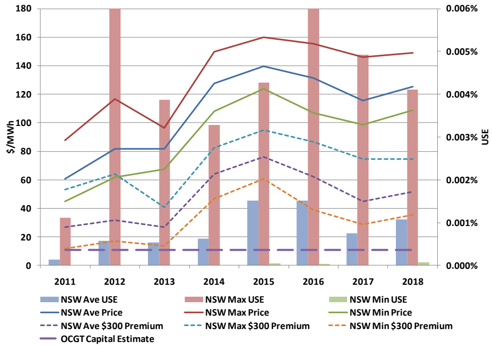
Figure 8-9 NSW 10 PoE Projections
