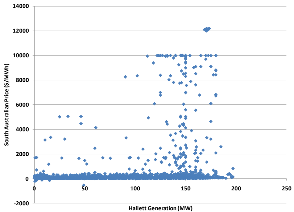
Figure 17-2 Hallett Generation versus Spot Price: 2006-2011
