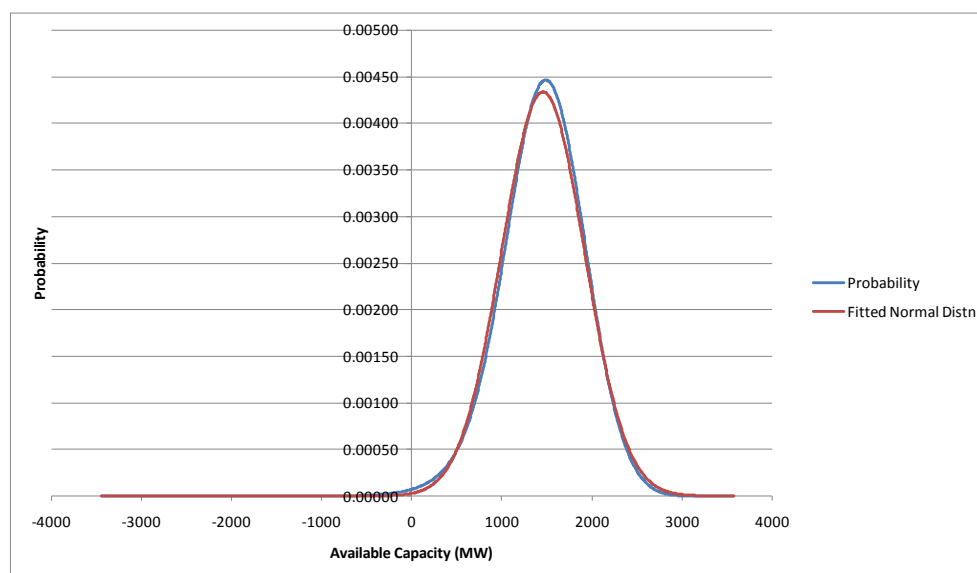
Figure 14-6 Probability Distribution of Generation Reserves
