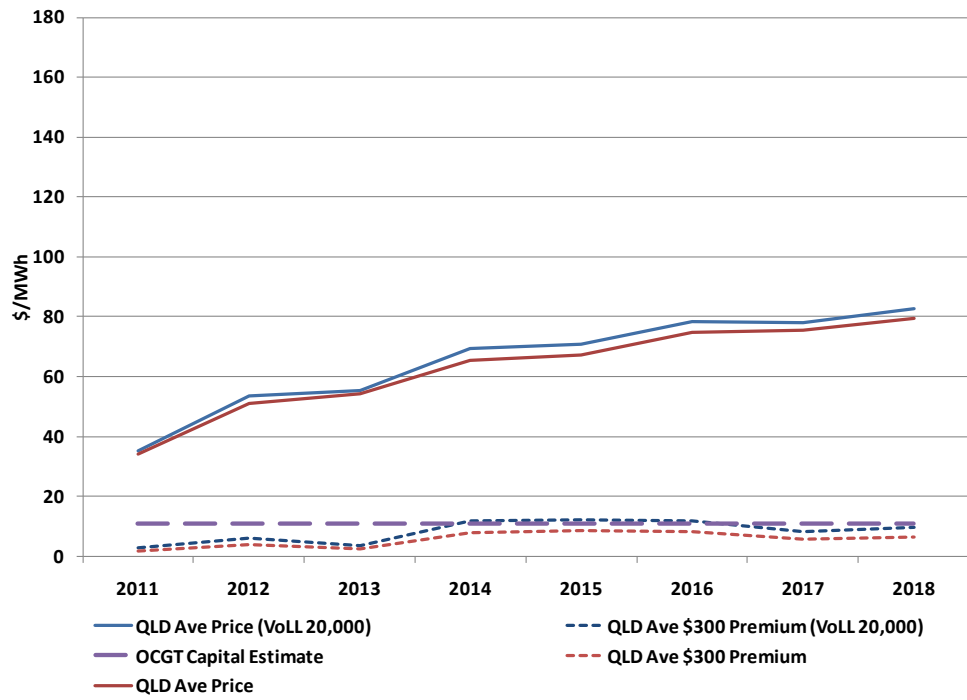
Figure 8-15 QLD Comparison
