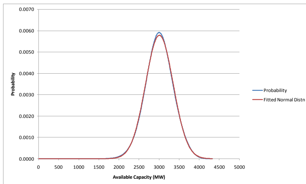
Figure 14-5 Probability Distribution of Combined Thermal and Wind Generation
