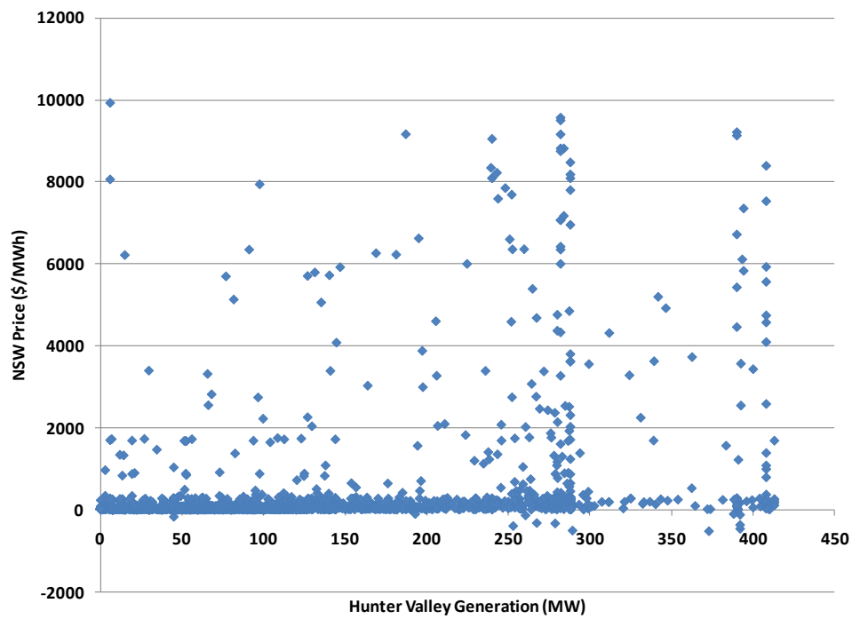
Figure 17-4 Hunter Valley Generation versus Spot Price: 2006-2011
