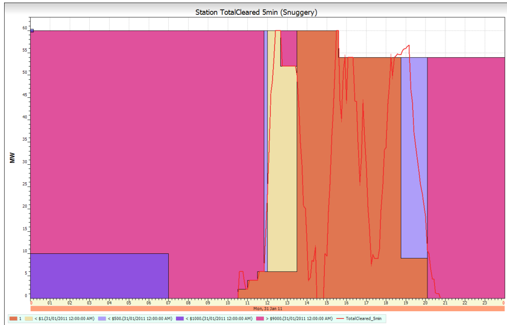
Figure 11-2 Snuggery Bids
