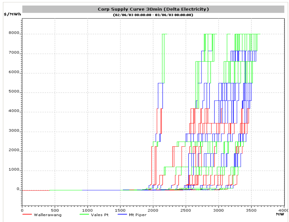
Figure 7-1 Typical Regional Supply Curve
