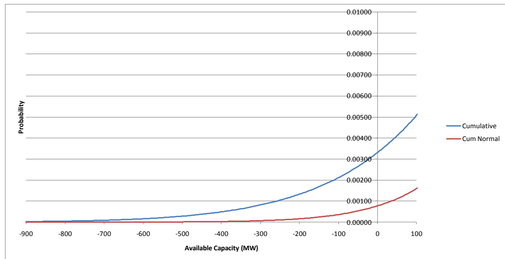
Figure 14-8 Cumulative Distribution of Reserves for Low Reserves
