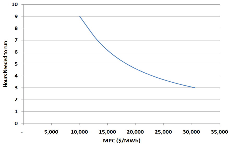
Figure 6-1 No Hours of OCGT Operation versus MPC
