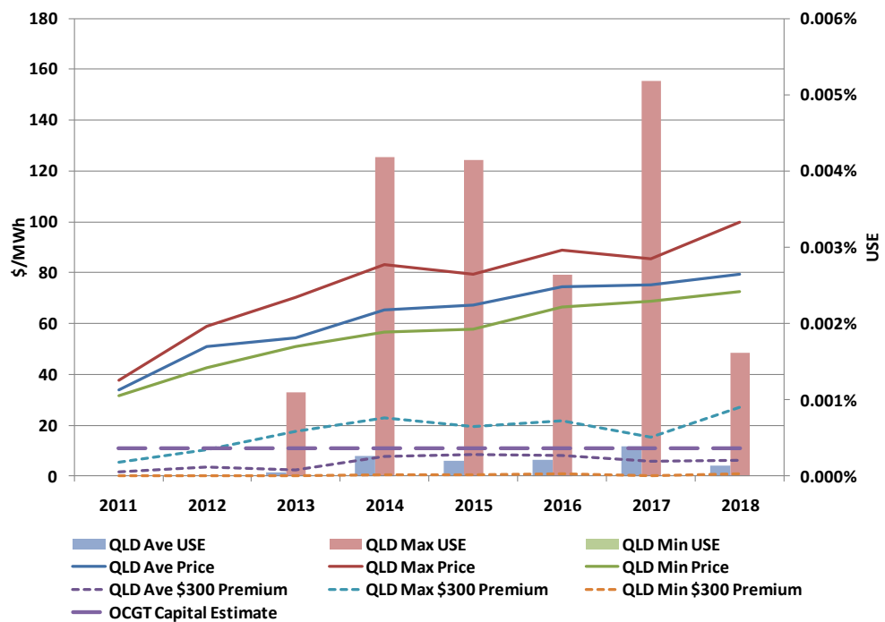
Figure 8-6 QLD 50 PoE Projections
