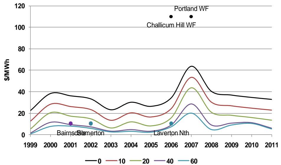
Figure 10-4 NEM New Entry – Victoria
