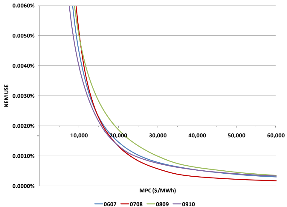
Figure 6-9 USE v MPC Relationship in the NEM
