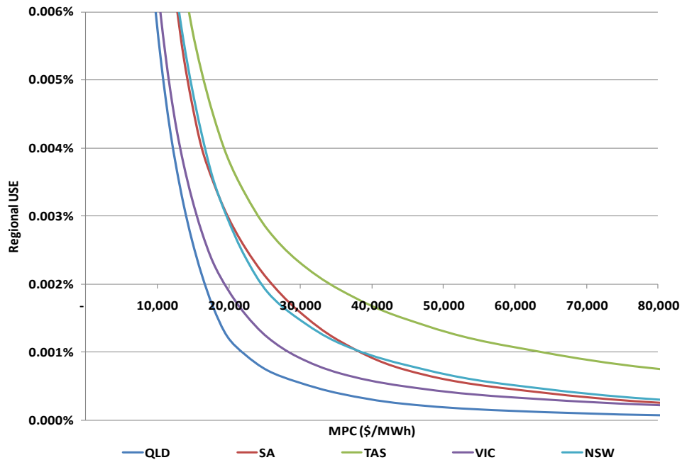
Figure 6-3 MPC v USE Relationship – 2008/09 Load Shape
