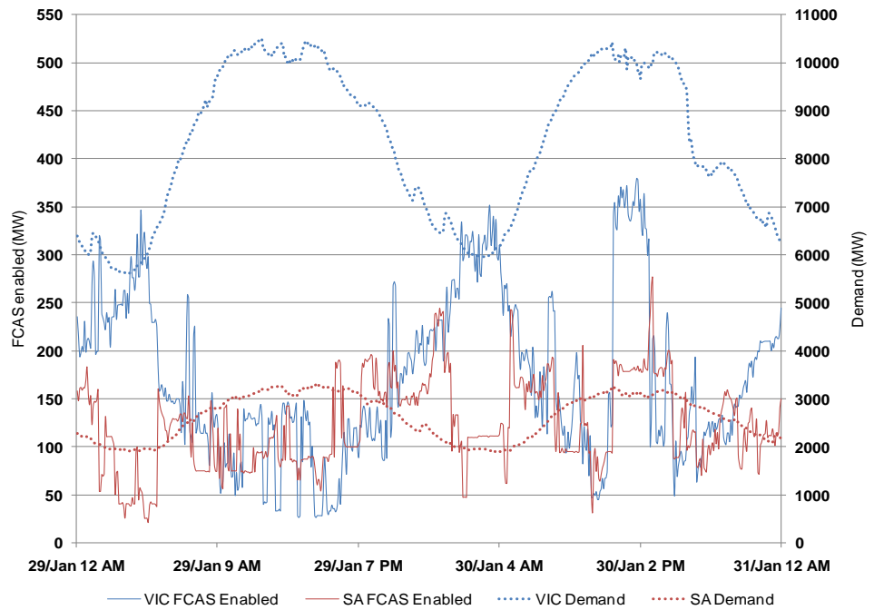
Figure 12-4 SA and Vic Demand, and FCAS Enabled
