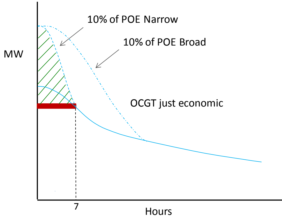
Figure 6-6 Extreme Peaking Plant Operation and 50% and 10% PoE Demands
