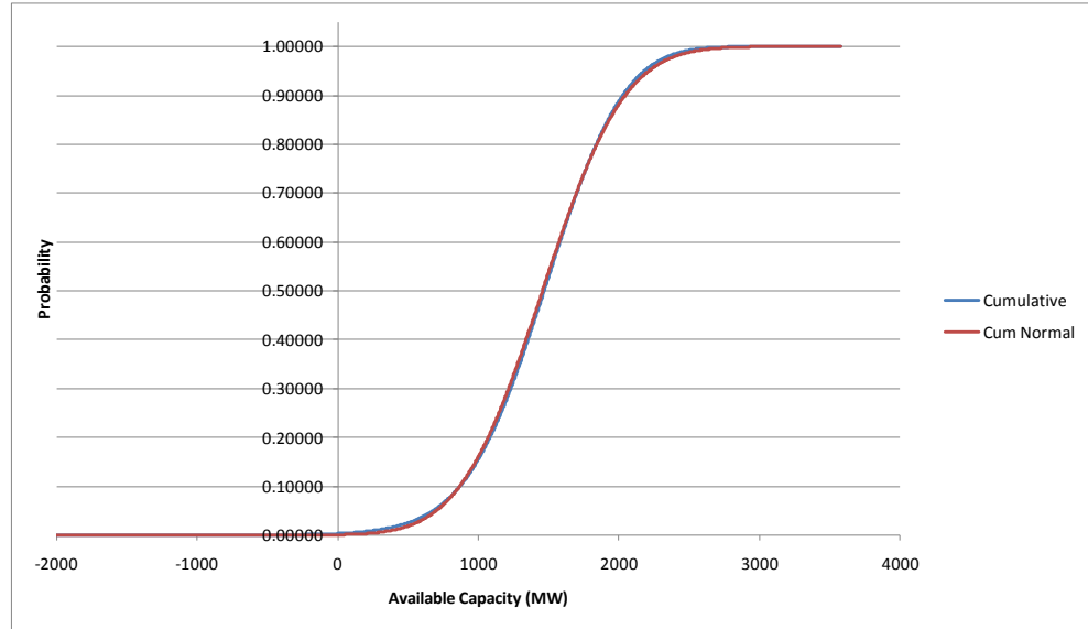
Figure 14-7 Cumulative Distribution of Reserves
