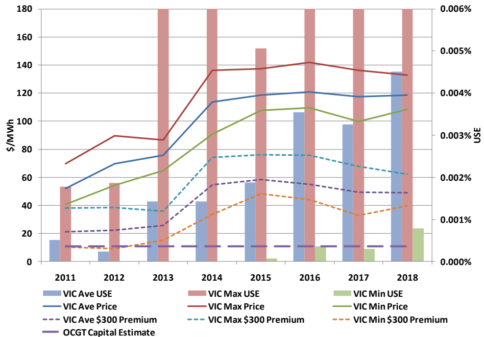
Figure 8-12 VIC 10 PoE Projections
