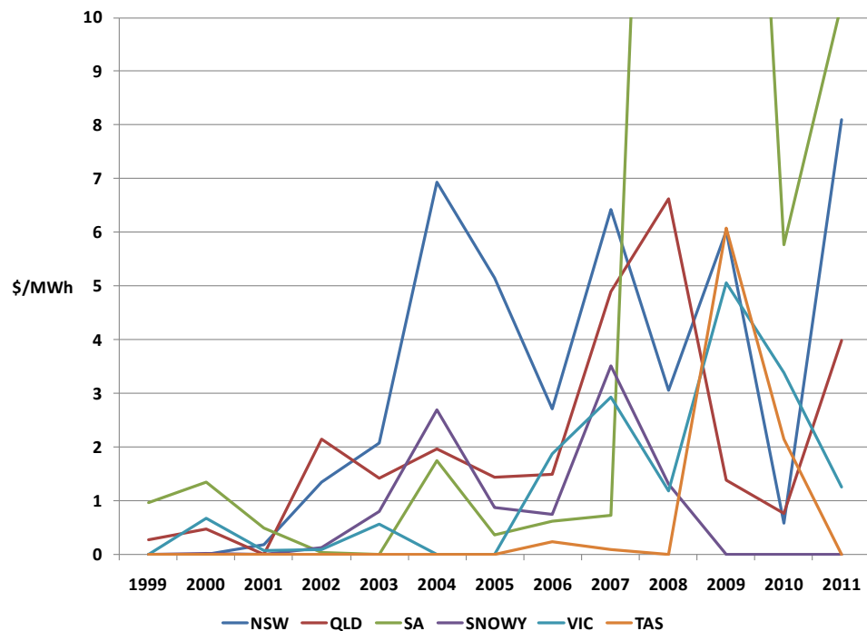
Figure 7-3 Historical Assessment of the Increase in Spot Price due to increasing the MPC to $20,000/MWh
