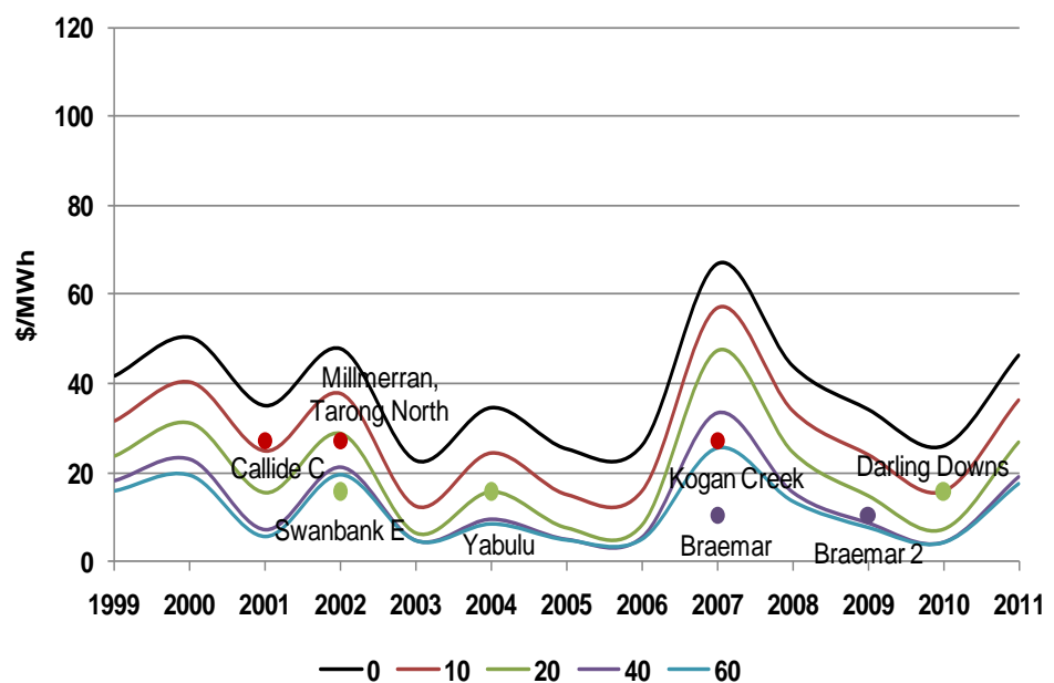
Figure 10-2 NEM New Entry – Queensland
