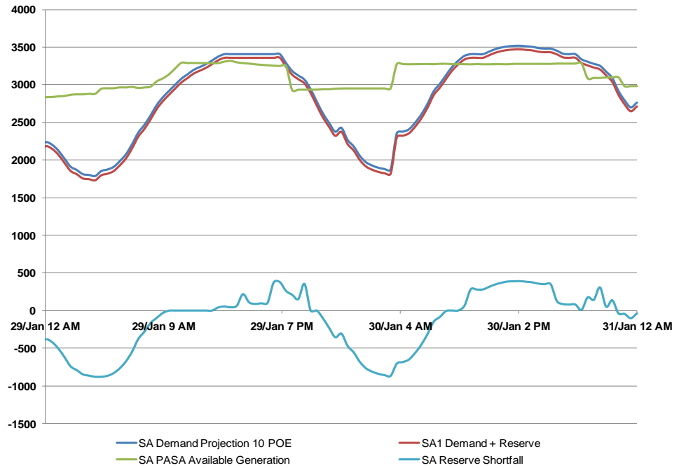
Figure 12-3 ST PASA Projection for SA – 29 and 30 January 2009
