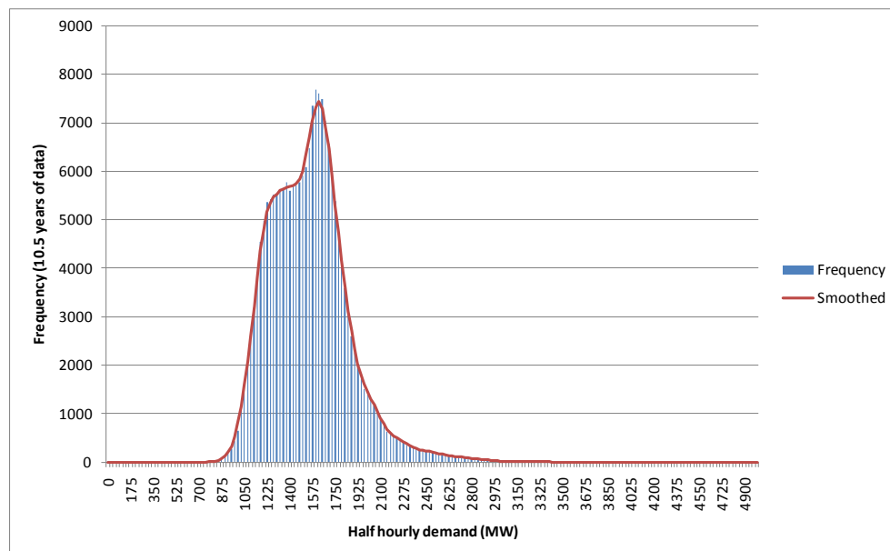
Figure 14-4 Frequency Distribution for Half Hourly SA Demand Data for 10½ years
