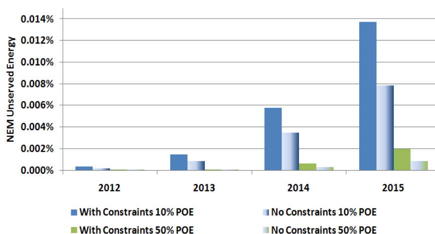
Figure 15-1 Sensitivity of Reliability to Inclusion of Intra-regional Constraints
