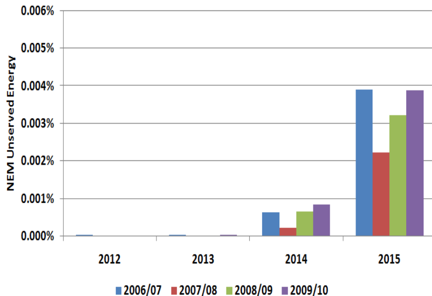
Figure 6-5 Reliability Sensitivity to Different Load Patterns
