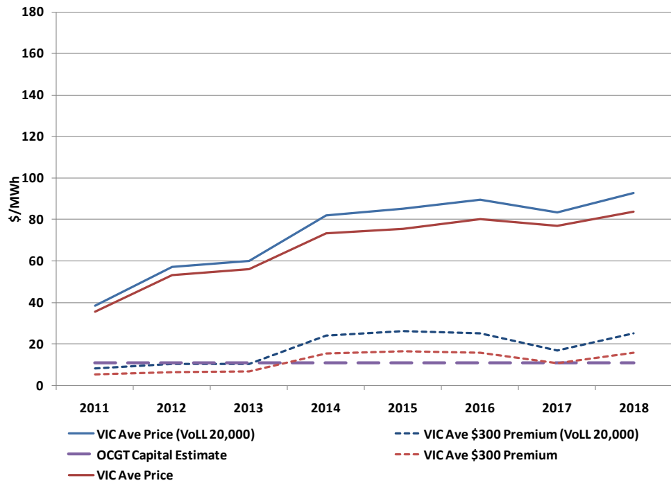
Figure 8-17 VIC Comparison
