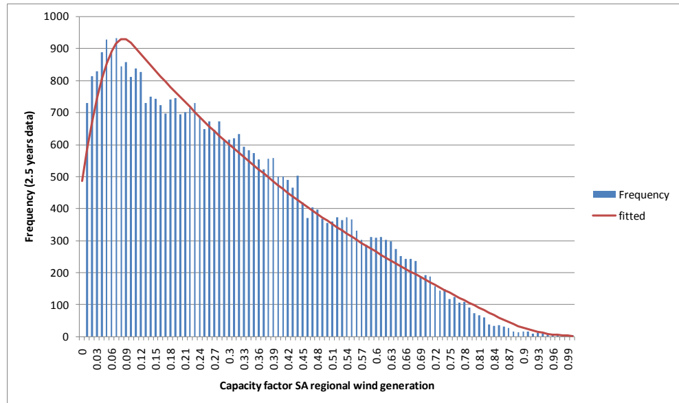
Figure 14-3 Frequency Distribution of SA Wind Generation Output in terms of Capacity Factor
