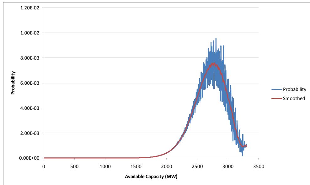
Figure 14-1 Distribution of Available Thermal Generation in SA
