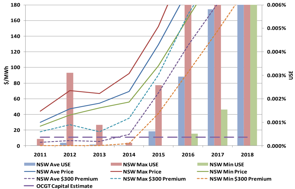
Figure 8-1 NSW 50 PoE No New Entry
